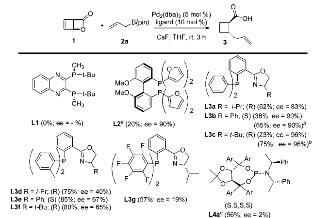
Scheme 2. Ligand Screening for the Catalytic Asymmetric Allylation
