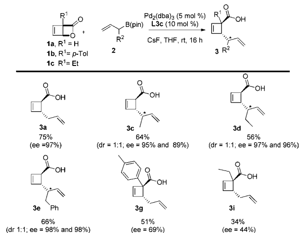
Scheme 3. Scope of Asymmetric Pd-Catalyzed Allylation of Lactones 1a–c a
