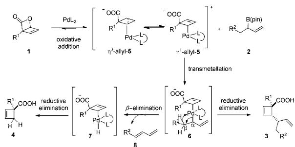
Scheme 4. Proposed Mechanism for the Catalytic Allylation
